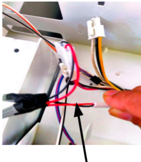
Wire Harness Connection
